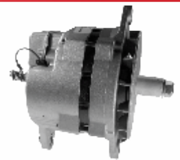
CLAVE: A01305 NO. PARTE: 110-555 ALTERNADOR RCP MOTOROLA 130A PRESTOLITE NUEVO 12V. CATERPILLAR, CHEV / GMC TRUCK FORD TRUCK TRUCK, FREIGHTLINER, IHC TRUCK, KENWORTH, NAVISTAR USA 1-2429-00MO LESTER 8058 8LHA2070V
